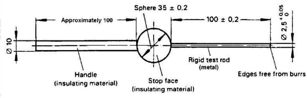
Dimensions in millimetres
