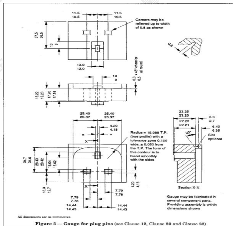
Figure 5 — Gauge for plug pins (see Clause 12, Clause 20 and Clause 22)
