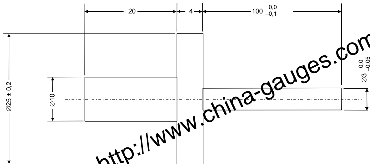
Figure C.4 – 100 mm × 3 mm test pin
