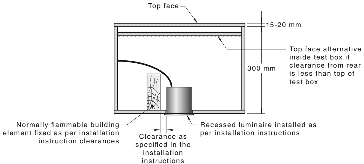
FIGURE ZA3 TEST BOX WITH FALSE CEILING TO MANUFACTURER’S INSTRUCTIONS
