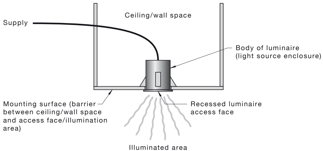
FIGURE ZC1 GENERAL PARTS OF A RECESSED LUMINAIRE
