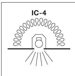
FIGURE 106 REQUIRED SYMBOL FOR IC-4 LUMINAIRES
