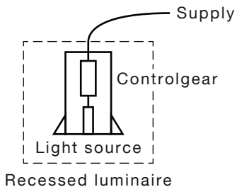
FIGURE ZC5 RECESSED LUMINAIRE WITH SUPPLIED COMPONENT PART CONTROLGEAR WITHIN ENCLOSURE OF LIGHT SOURCE
