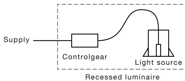
FIGURE ZC3 RECESSED LUMINAIRE WITH SUPPLIED COMPONENT PART CONTROLGEAR CONNECTED BY INTERCONNECTING CORD TO LIGHT SOURCE
