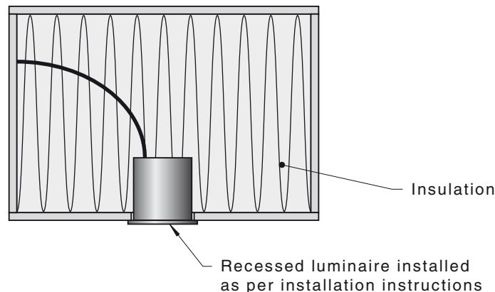
FIGURE ZA6 TEST SET-UP FOR ABNORMAL OPERATION FOR DO-NOT-COVER, CA90 AND CA135 AND NORMAL OPERATION FOR IC AND IC-4 LUMINAIRES
