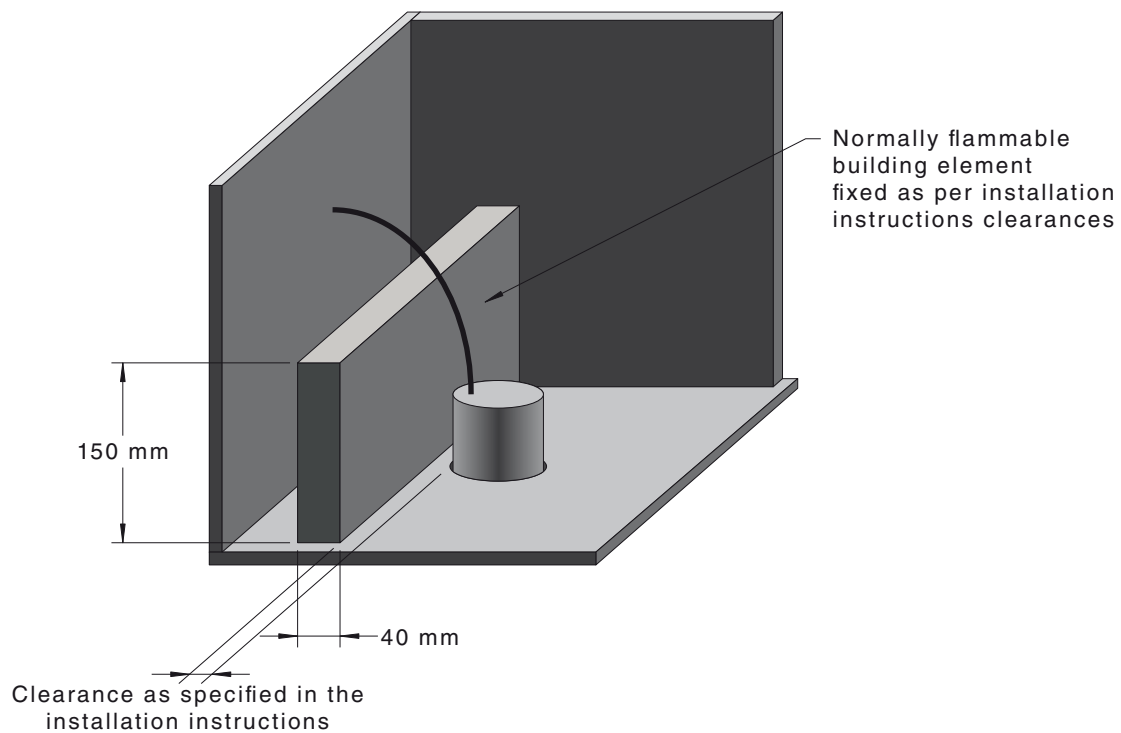
FIGURE ZA2 TEST BOX WITH SIMULATED BUILDING ELEMENT (WITH FRONT, SIDE AND TOP REMOVED)
