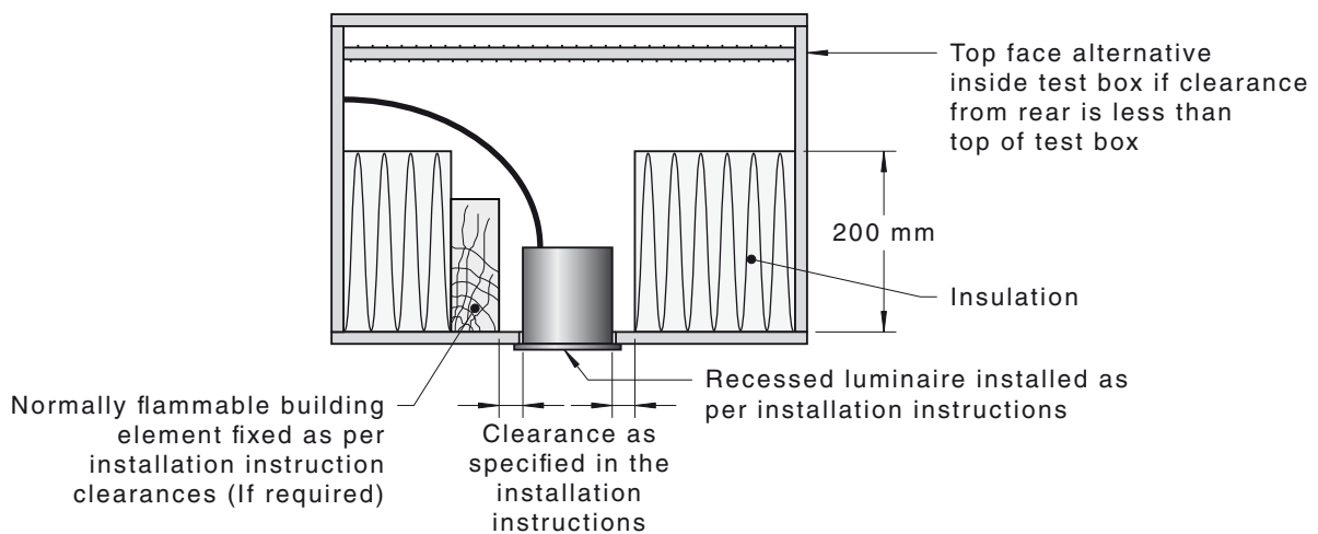
FIGURE ZA4 TEST SET-UP FOR DO-NOT-COVER LUMINAIRES
