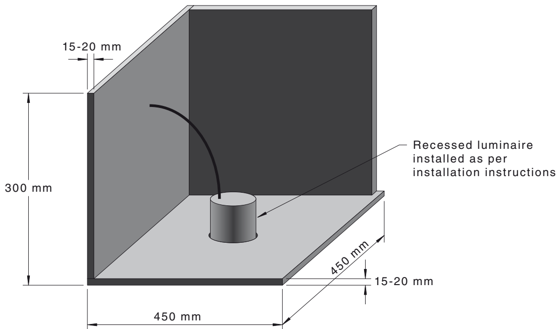
FIGURE ZA1 TEST BOX (WITH FRONT, SIDE AND TOP REMOVED)
