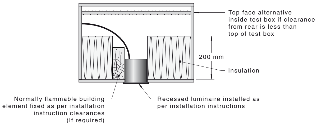
FIGURE ZA5 TEST SET-UP FOR CA90 AND CA135 LUMINAIRES
