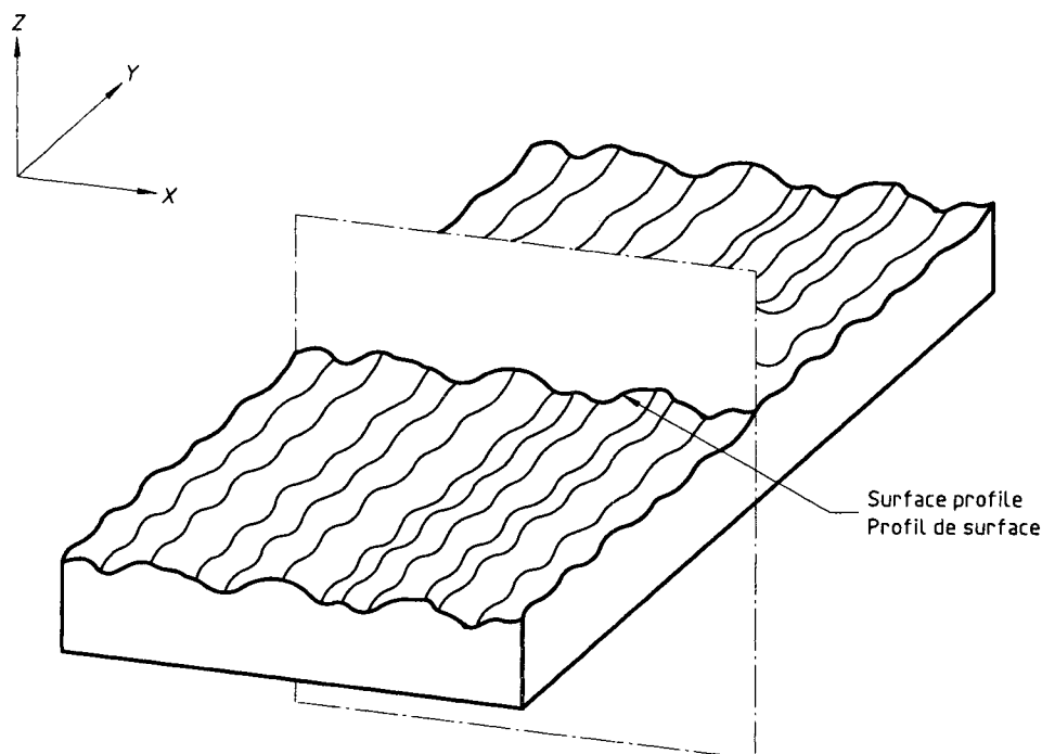
Figure 2 — Surface profile Figure 2 — Profil de surface
