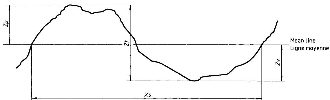
Figure 3 — Profile element Figure 3 — Élément du profil
