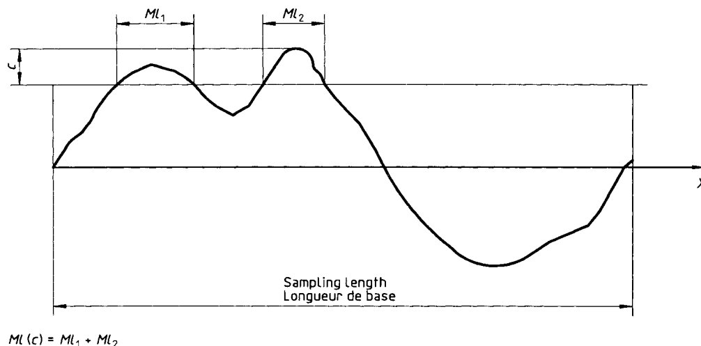
Figure 5 — Material length Figure 5 — Longueur portante
