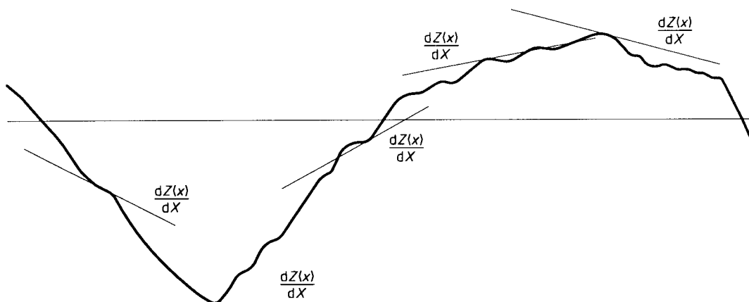
Figure 4 — Local slope Figure 4 — Pente locale
